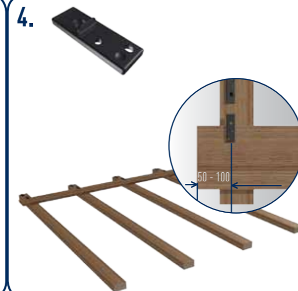
2 x BohrFix® FB
