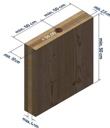
Vertical manipulation of CLT
