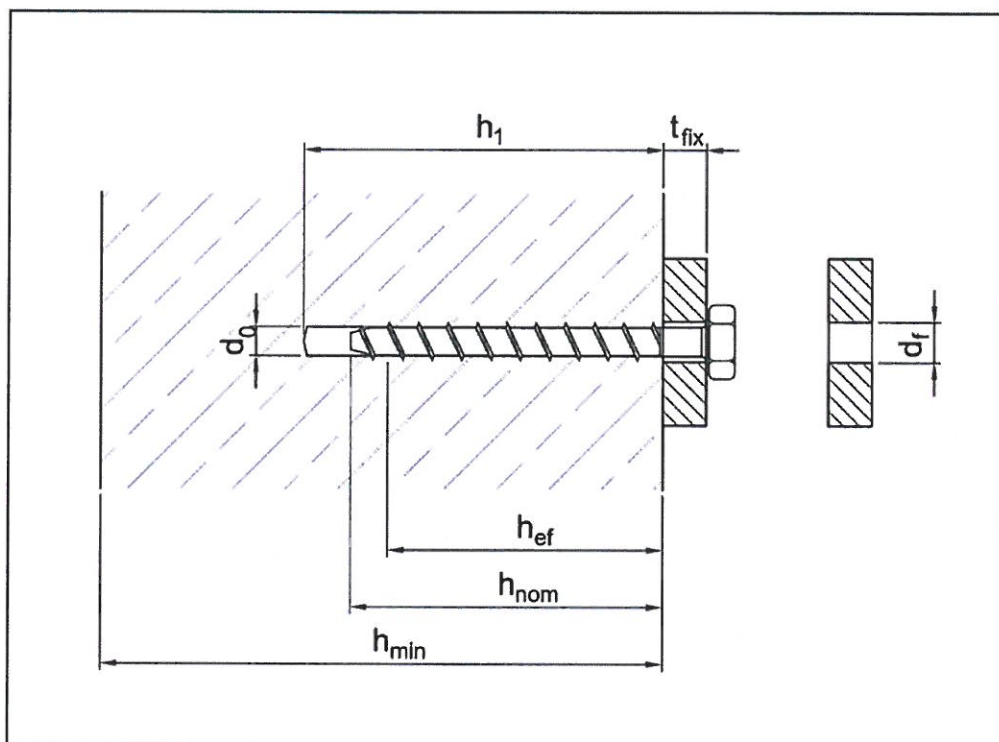
BeziFix Anker hexagon head and hexagon head with flange: sizes 7,5, 10,5 and 12,5
