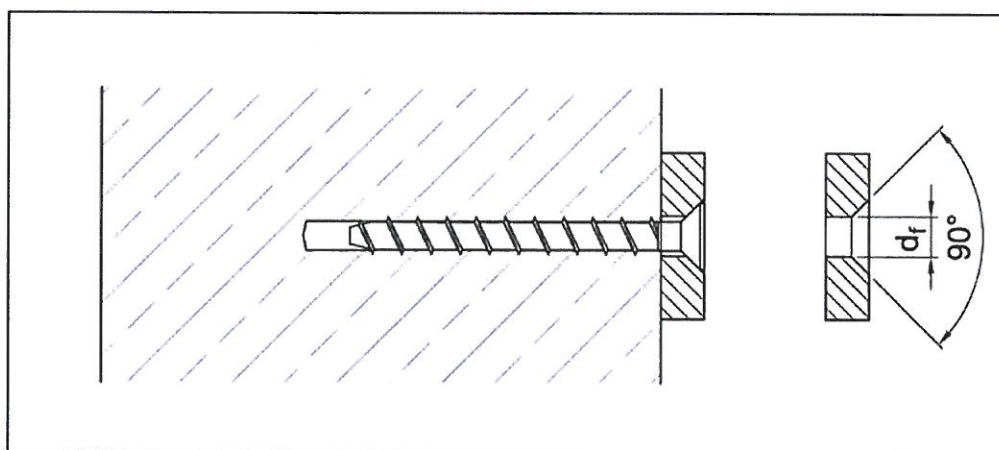
BeziFix Anker countersunk head: size 7,5
