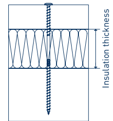
Soft insulating materials (compressive stress at 10 % compression under 50 kPa)
